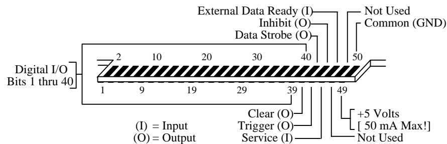
Digital488 Rear Panel I/O Connector Pin Out
